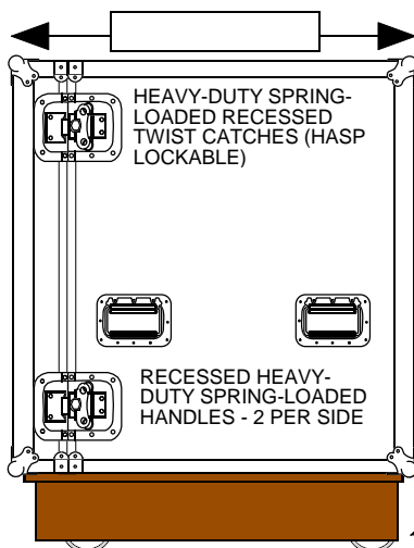
SIDE VIEW-CASE CLOSED
