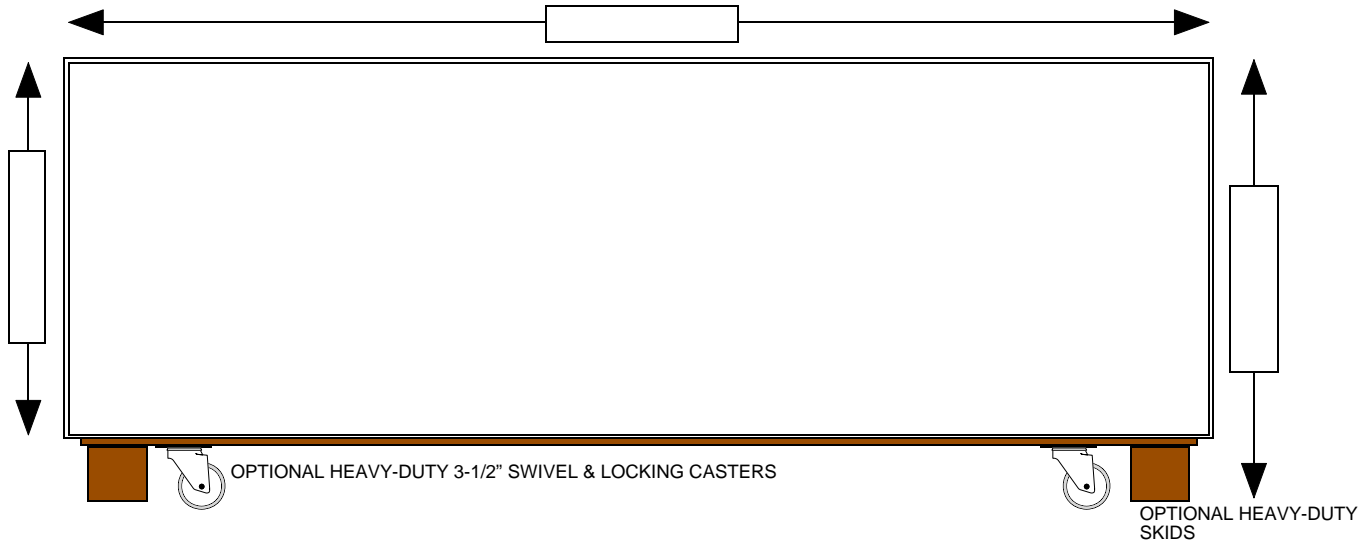
CASE FRONT REMOVABLE LID-REMOVED-SHOWING OPTIONAL COLLAPSIBLE TABLE LEGS
