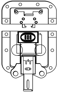
Recessed Twist/Combination Lock Assembly
