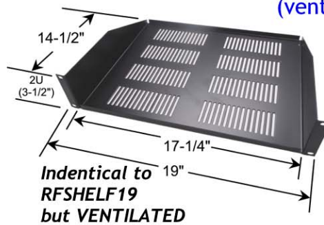
RFSHELF17SLV (ventilated)
