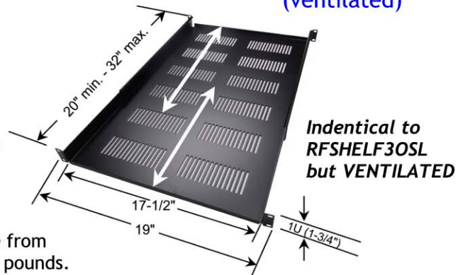
RFSHELF30SLV (ventilated)
